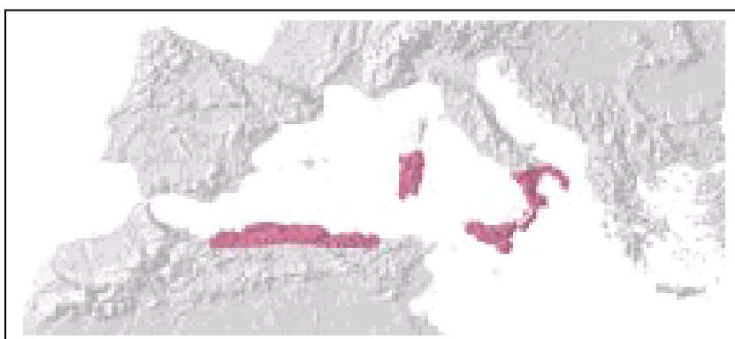
Fig. 3. Distribution map of Ambrosina bassii L. (From Mayo et al. 1997). Genera of Araceae (1997) does not indicate the species for Corsica.
