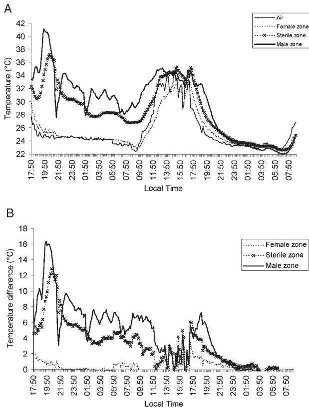
Figure 2. A. Temperature curves (°C) of the male zone, the sterile male zone, the female zone, and the ambient air during two days of flowering for P. solimoense . B. Curves of differences in temperature (°C) between the male zone, the sterile male zone and the female zone, and the ambient air during two days of flowering for P. solimoense . The fluctuations of temperature during the afternoon of the second day (13–17 h) are due to the presence of frequent and intermittent rains.
