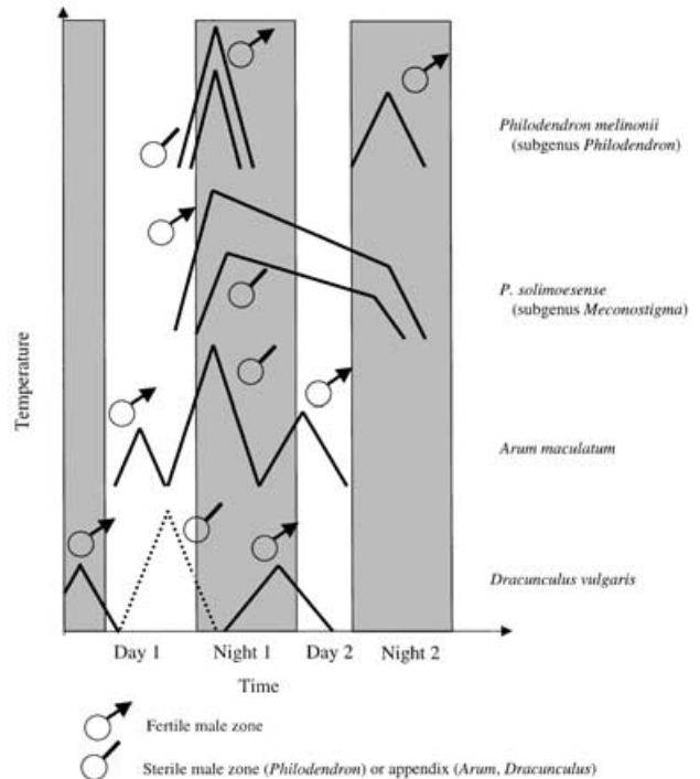
Figure 3. Schematic representation of the thermogenetic cycles of Arum maculatum (Bermadinger-Stabentheiner & Stabentheiner, 1995), Dracunculus vulgaris (Seymour & Schultze-Motel, 1999), P. melinonii and P. solimoense (this study). The first day is the time when the insects arrive at the inflorescence.
