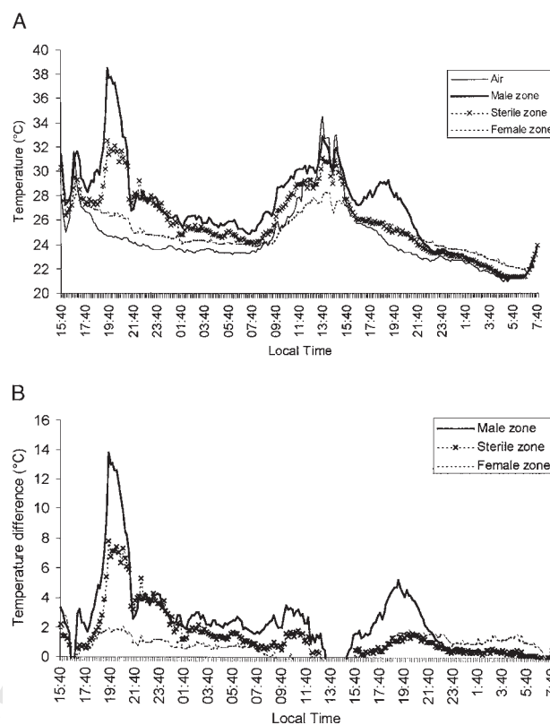
Figure 1. A. Temperature curves (°C) of the male zone, the male sterile zone, the female zone, and the ambient air during two days of flowering for P. melinonii . B. Curves of differences in temperature (°C) between the male zone, the sterile male zone and the female zone, and the ambient air during two days of flowering for P. melinonii .
